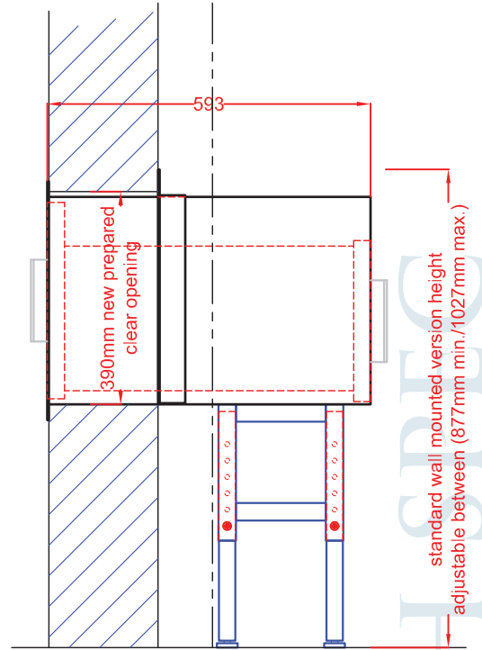
SECTIONAL VIEW
